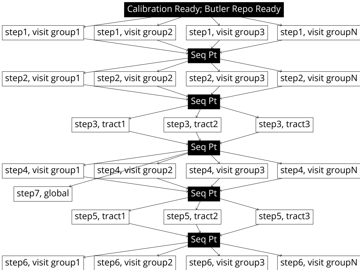
FIGURE 1: Illustration of the high level DRP workflow for DP0.2. Each white box represents a BPS submission which is a workflow on its own. Typically each submission runs a quantum graph of tens of thousands quanta.
